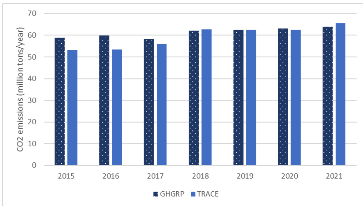
Figure 6 U.S. GHGRP (dark blue bars with white dots) adjusted and TRACE (light blue bars) emissions comparisons for years 2015 to 2021. 2021 is the most recent year with UNFCCC data.
