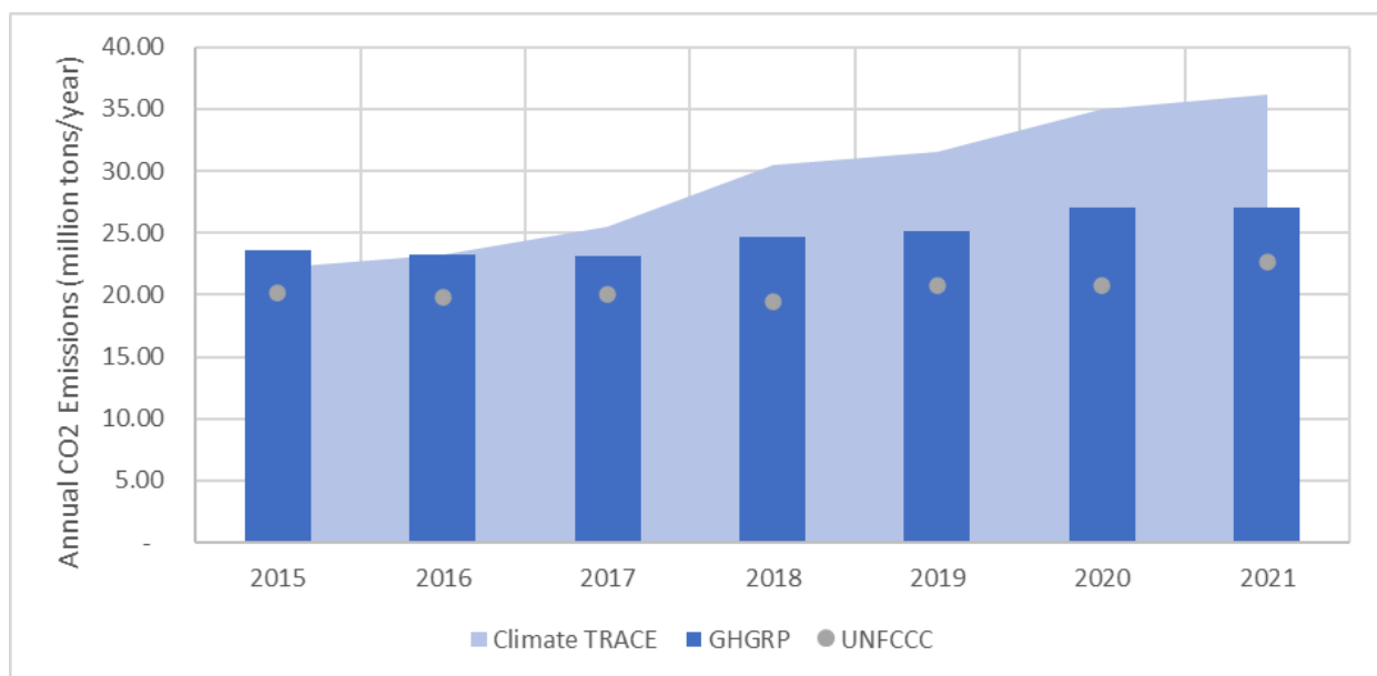
Figure 5 U.S. GHGRP, UNFCCC, and TRACE emission comparisons for years 2015 to 2021. 2021 is the most recent year with UNFCCC data.
