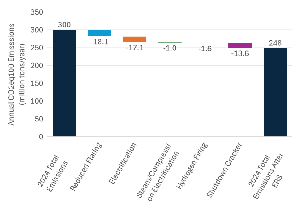
Figure 8 Waterfall chart demonstrating share of total emissions reductions achieved for each ERS lever. Assets employing specific strategies in this figure don't necessarily match what is employed on the Climate TRACE website.
