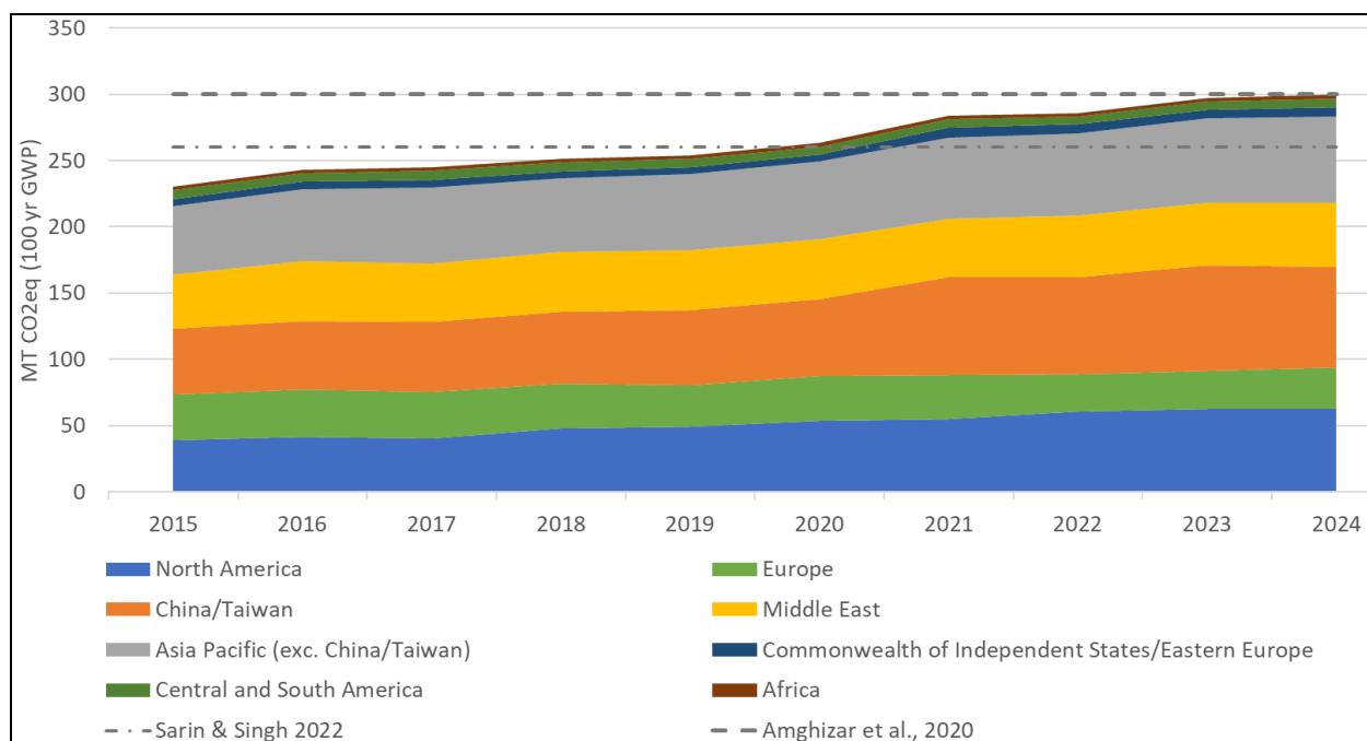
Figure 3 Climate TRACE emission estimates by region. Each region contains the following countries- North America (light blue): Canada, U.S., and Mexico; China/Taiwan (orange); Asia Pacific exc. China/Taiwan (gray): Australia, India, Indonesia, Japan, Malaysia, Philippines, Singapore, South Korea, and Thailand; Central and South America (dark green): Argentina, Brazil, Colombia, and Venezuela; Europe (light green); Austria, Bulgaria, Belgium, Croatia, Czech Republic, Finland, France, Germany, Greece, Hungary, Italy, Netherlands, Norway, Poland, Portugal, Romania, Slovakia, Spain, Sweden, Switzerland, Turkey, and United Kingdom; Middle East (yellow): Iran, Iraq, Israel, Kuwait, Oman, Qatar, Saudi Arabia, and United Arab Emirates; Commonwealth of Independent States/Eastern Europe (dark blue): Azerbaijan, Belarus, Russia, Serbia, Turkmenistan, Ukraine, and Uzbekistan; Africa (dark red): Algeria, Egypt, Libya, Nigeria, and South Africa.
